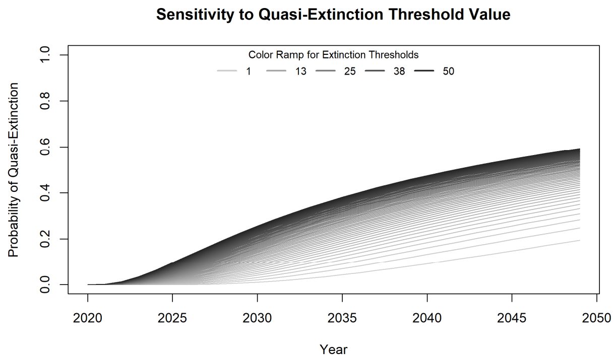
Figure 5: Sensitivity of the probability of quasi-extinction to the choice of starting abundance value (top) and quasi-extinction threshold (bottom). Grayscale lines represent a range of choices.
